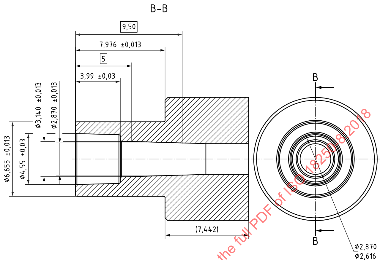
Figure C.4 — Female-insert APHERESIS AC RESERVOIR reference CONNECTOR, CONNECTOR used for leakage, separation from unscrewing and stress cracking test methods
