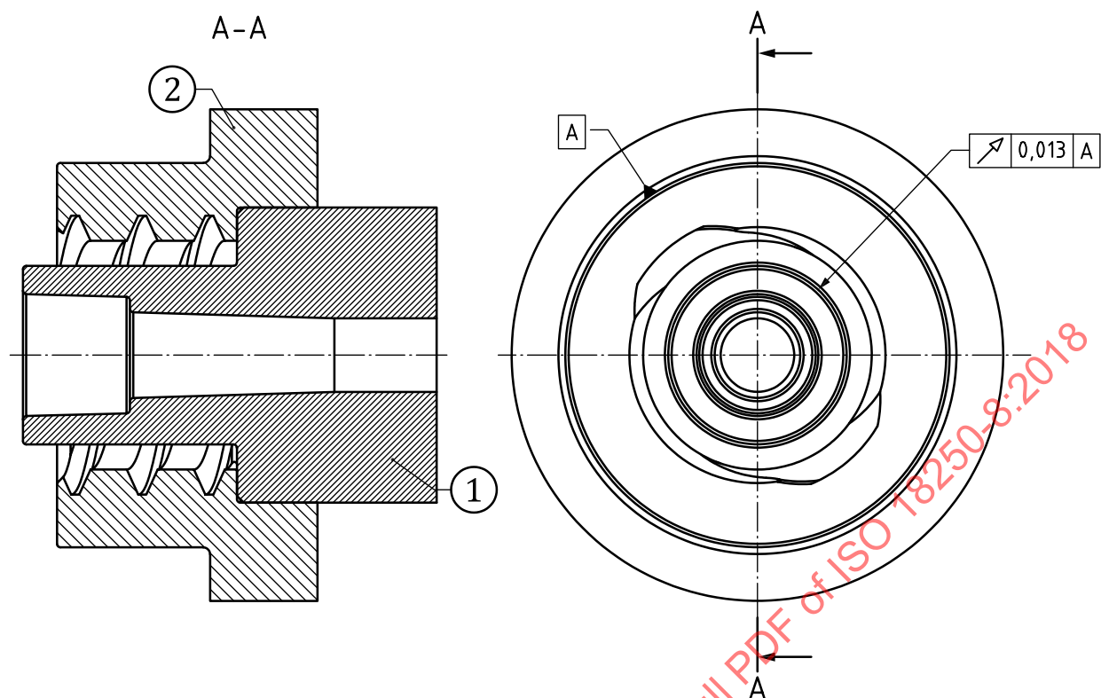
Figure C.6 — Female APHERESIS AC RESERVOIR reference CONNECTOR, CONNECTOR used for separation from axial load and resistance to overriding test methods
