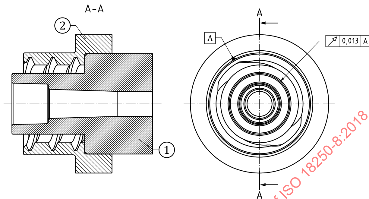
Figure C.2 — Female APHERESIS AC RESERVOIR reference CONNECTOR, CONNECTOR used for leakage, separation from unscrewing and stress cracking test methods
