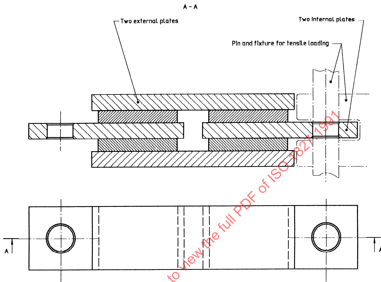
Figure 1 — Test piece arrangement
