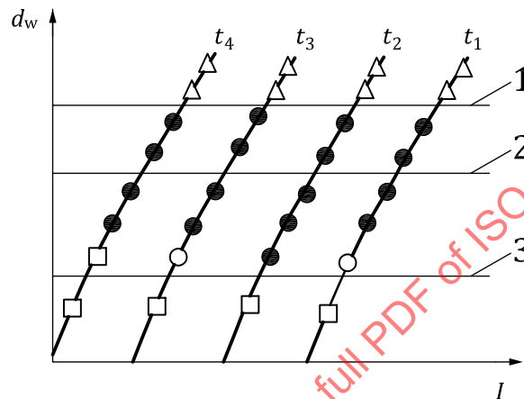
a) Welding current range diagram by constant electrode force and weld time t_1 < t_2 < t_3 < t_4
