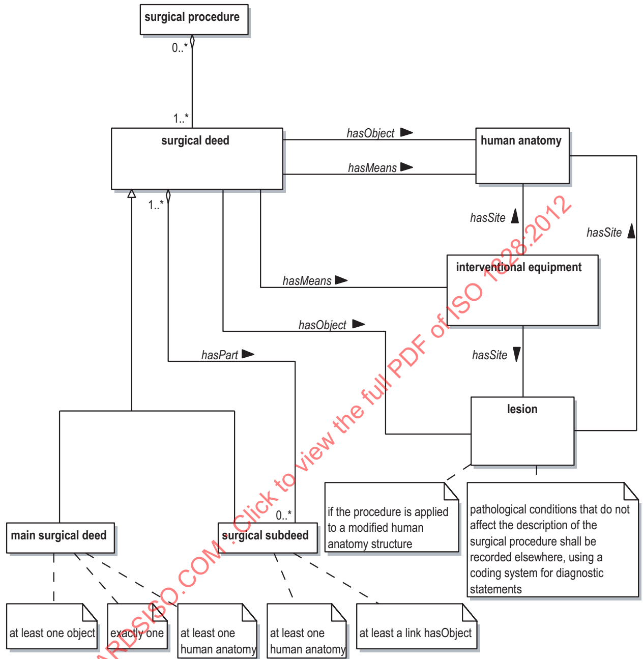
Figure 1 — UML diagram
