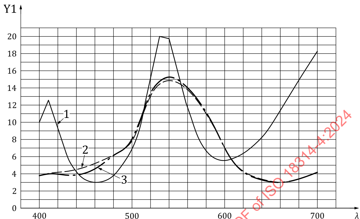
a) Reflectance functions of the standard Green-1, the sample Green-2 and corrected reflectance function of the sample Green-2 under the reference illuminant D65
