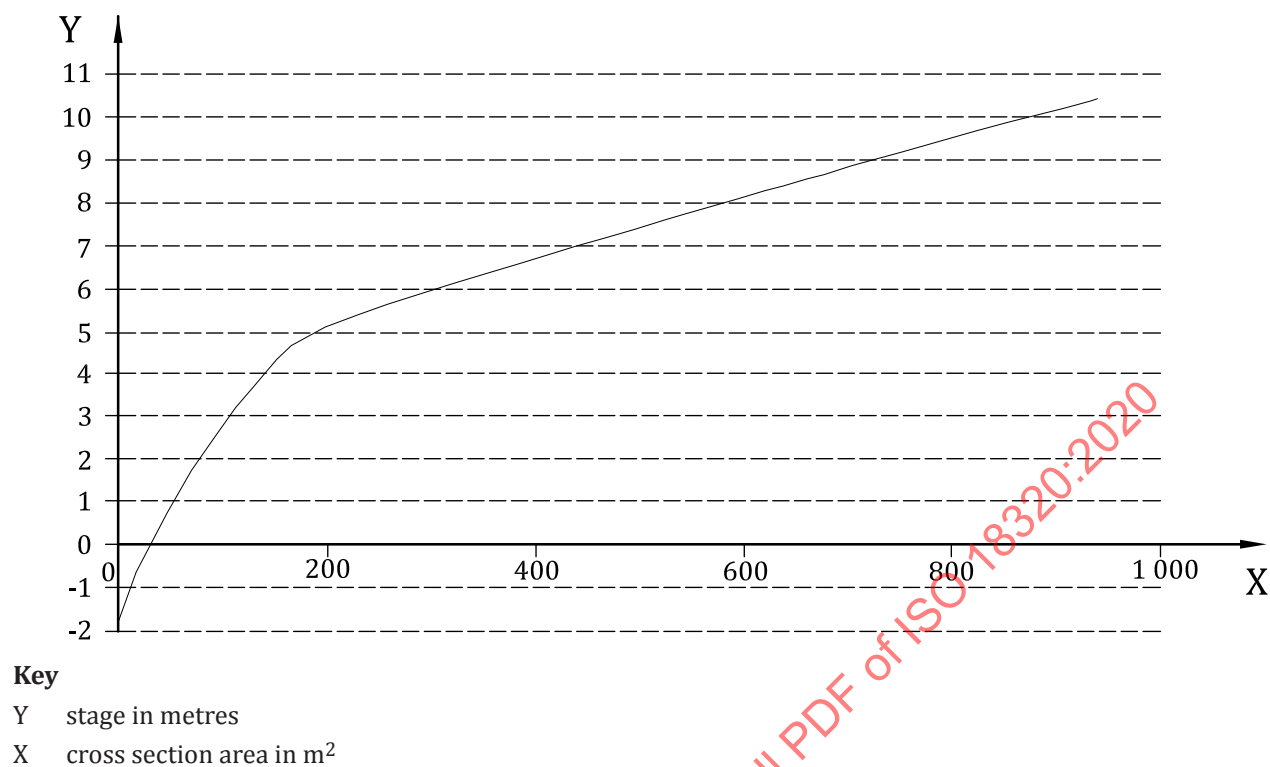
Figure E.4 — Variation of cross section area with stage, River Severn at Montford Bridge
