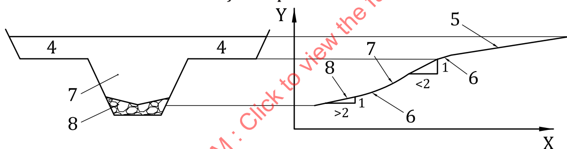
b) Flood plain added
