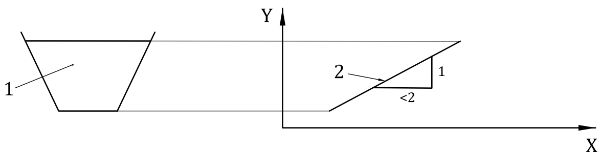
a) Trapezoidal channel with no flood plain and with channel-control conditions
