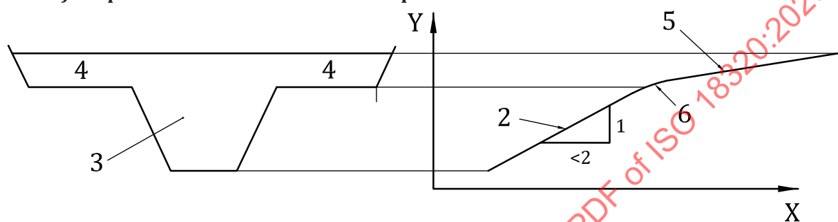
b) Flood plain added
