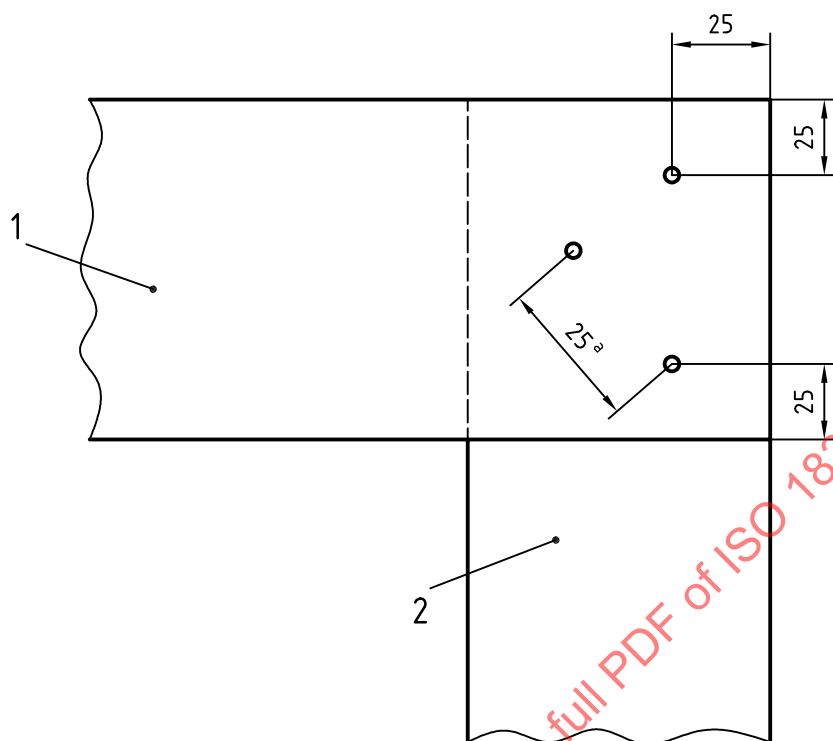
a) Example of nail spacing for block-type pallets
