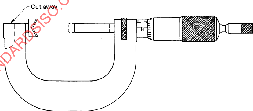
FIGURE 4 — Micrometer gauge
