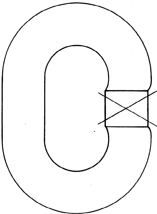
FIGURE 2 — Undercut at weld (not permissible)
