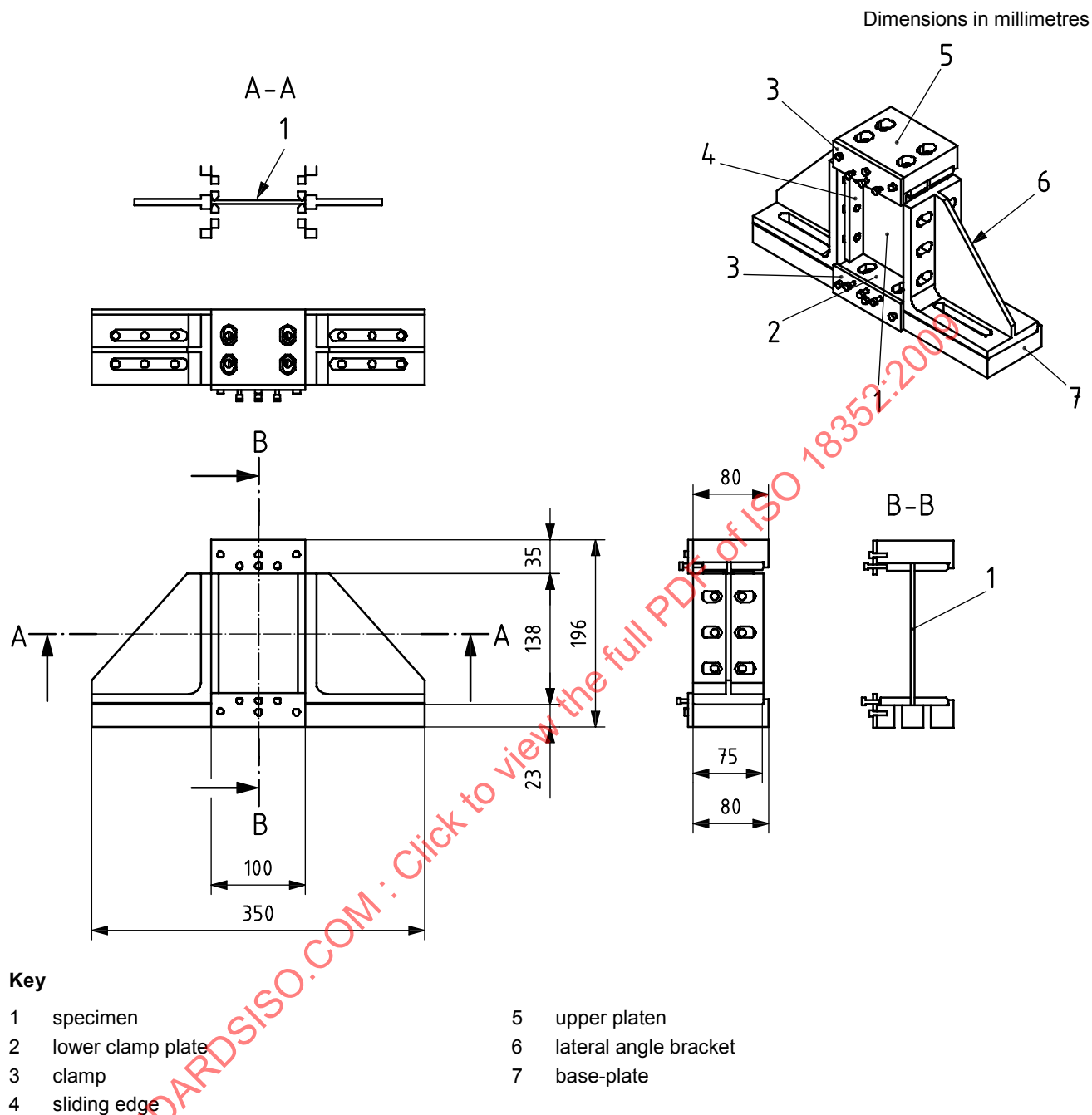
Figure 4 — Example of a compression-loading fixture
