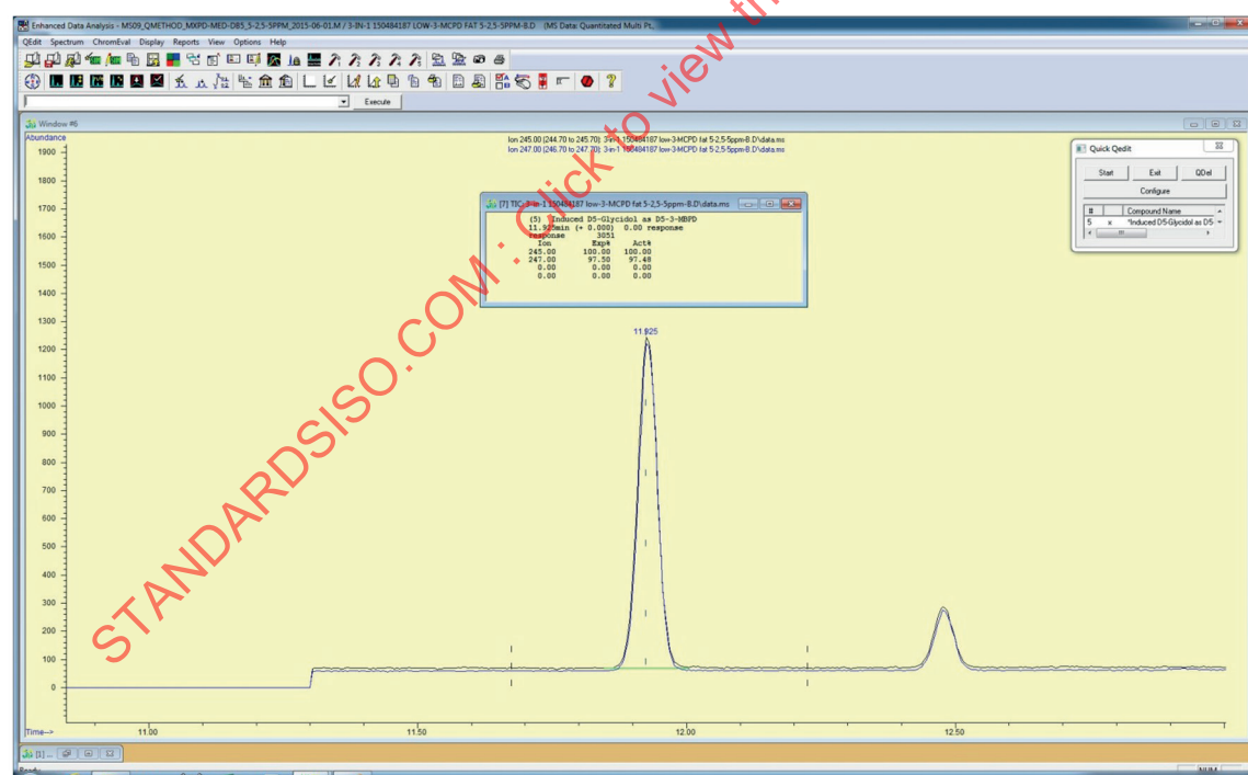
Figure A.9 — SIM — Chromatogram of glycidol-d 5 (for response determination) in assay B
