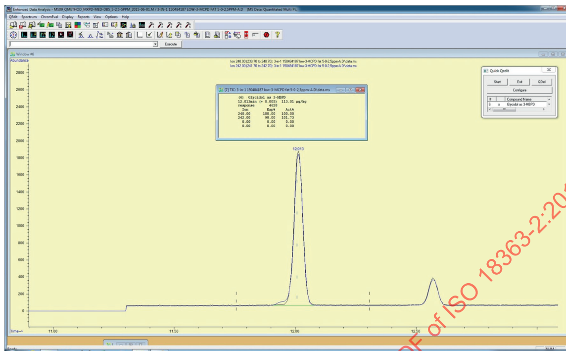
Figure A.4 — SIM — Chromatogram of glycidol (0.113 mg/kg) in assay A
