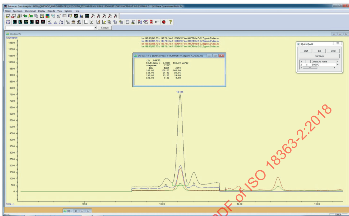
Figure A.2 — SIM — Chromatogram of 3-MCPD (0,155 mg/kg) in assay A
