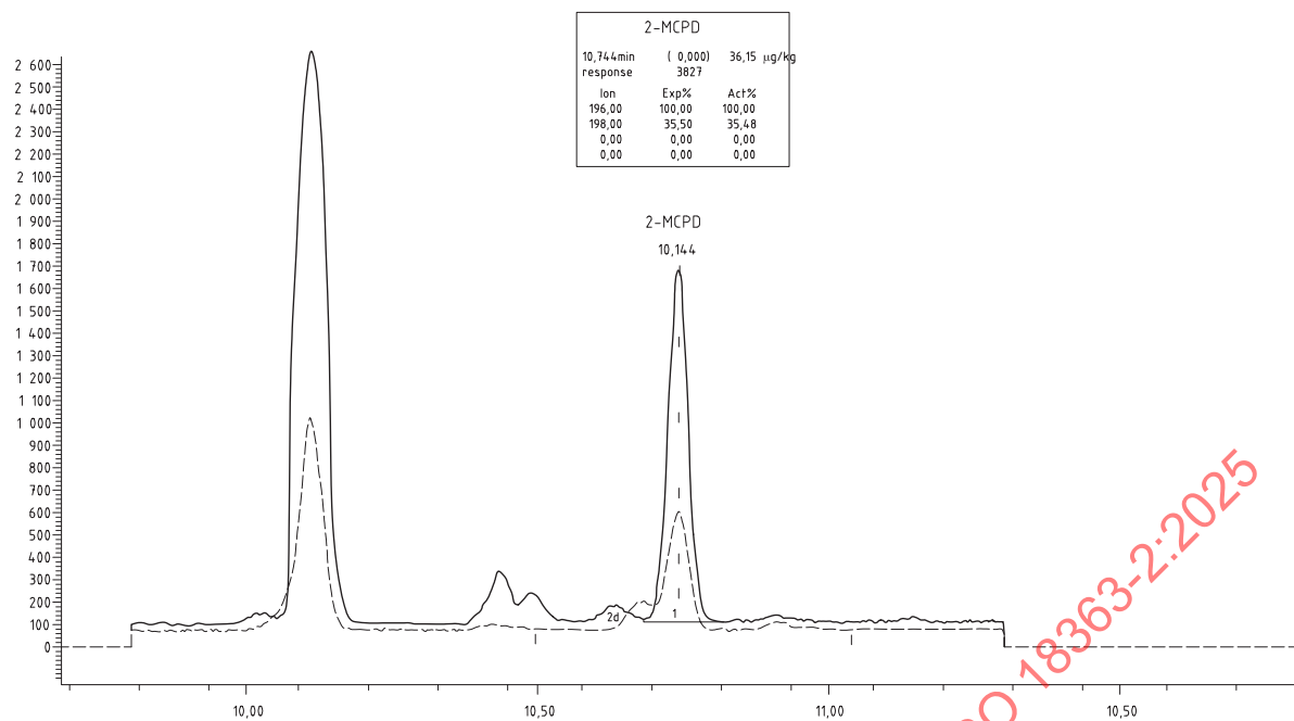
Figure A.8 — SIM — Chromatogram of 2-MCPD (0,036 mg/kg) in assay B
