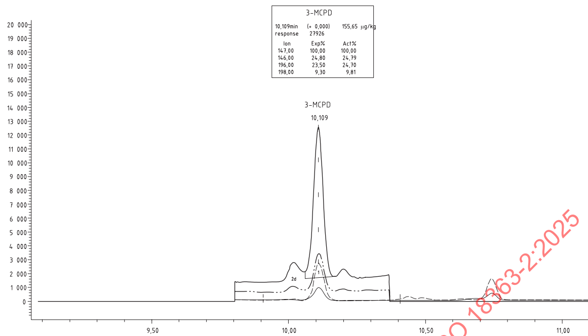
Figure A.6 — SIM — Chromatogram of 3-MCPD (0,156 mg/kg) in assay B
