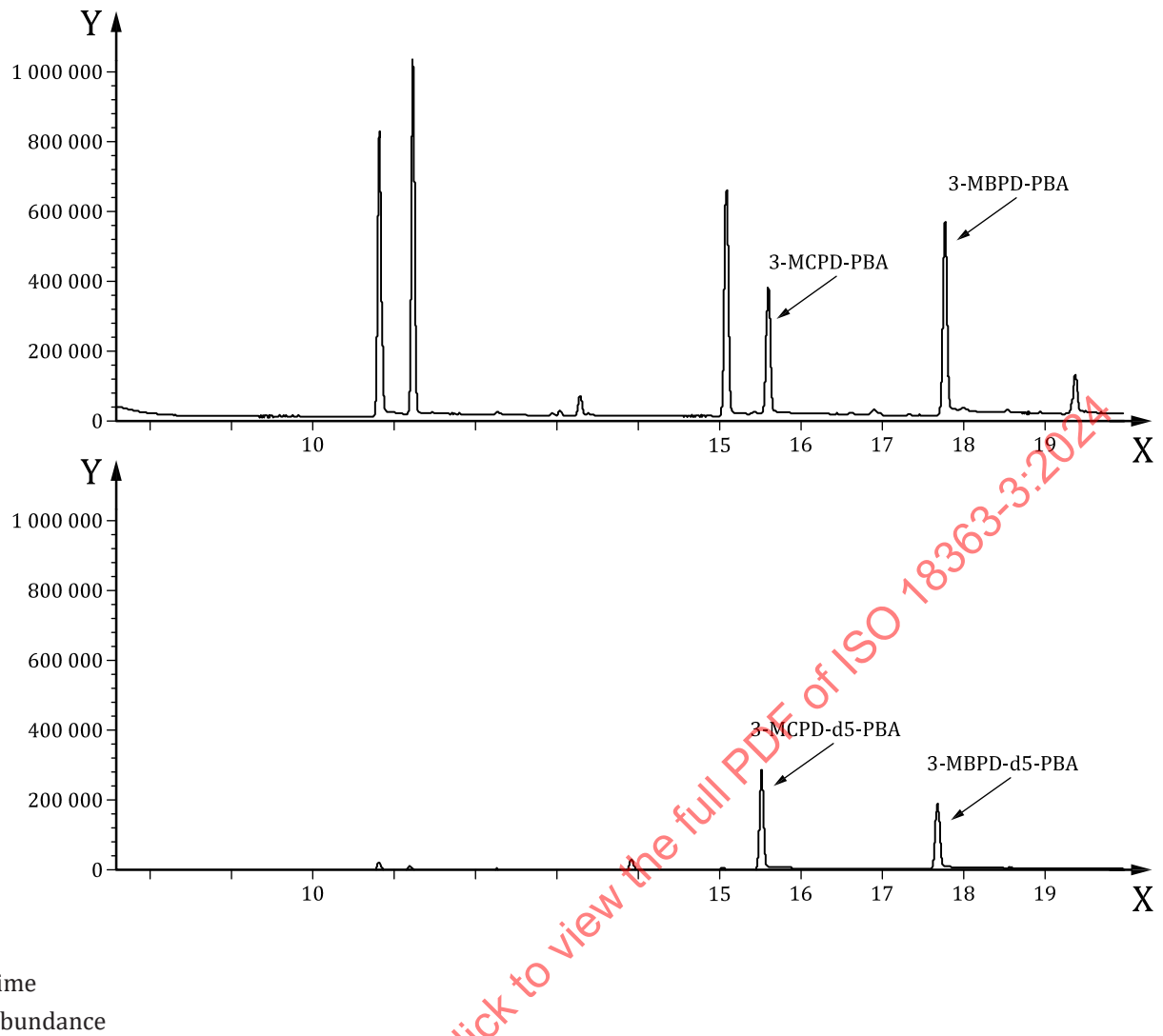
Figure A.3 — SIM chromatogram of a sample of fully refined palm oil (extracted ions m/z 147 and 150)
