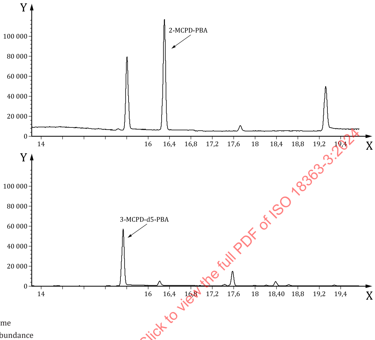
Figure A.4 — SIM chromatogram of a sample of fully refined palm oil (extracted ions m/z 196 and 201)
