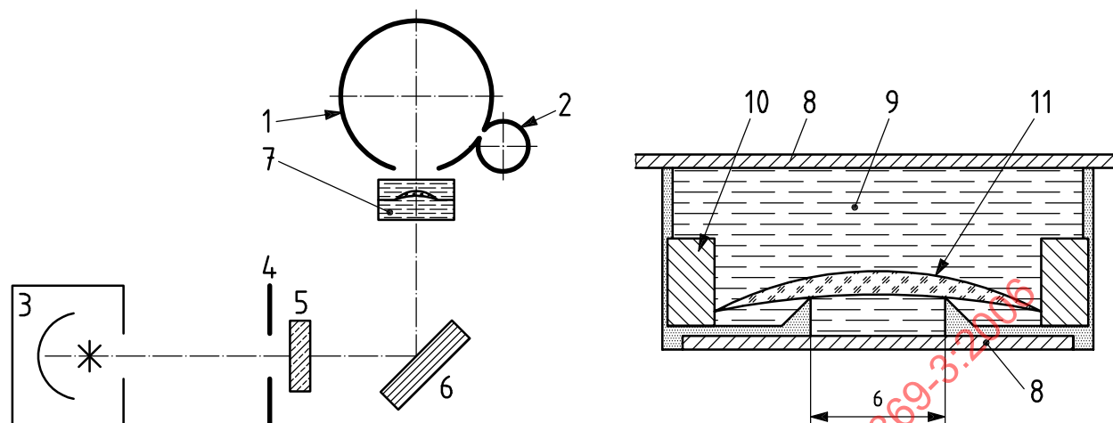
a) Apparatus for determination of spectral and luminous transmittance
