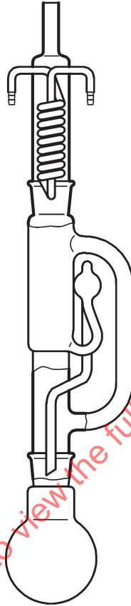
Figure 1 — Extraction apparatus
