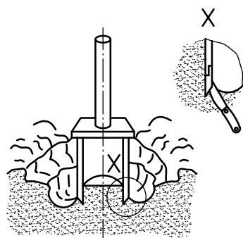
a) Positioning the sampler
