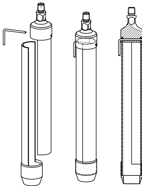
Figure C.9 — Split tube sampler
