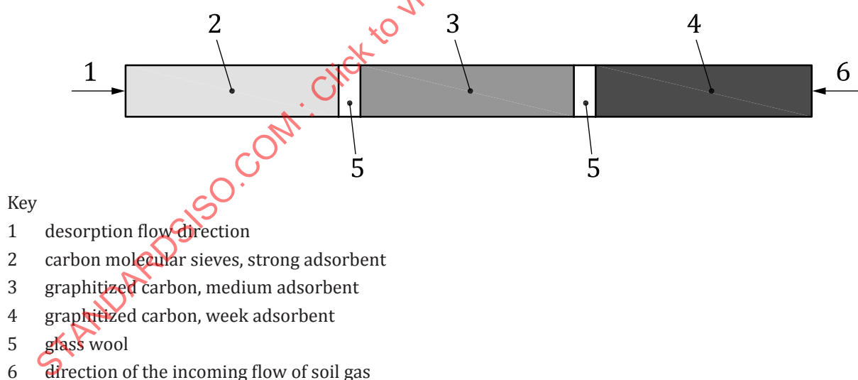
Figure 4 — Schematic representation of a multisorbent thermal desorption tube
