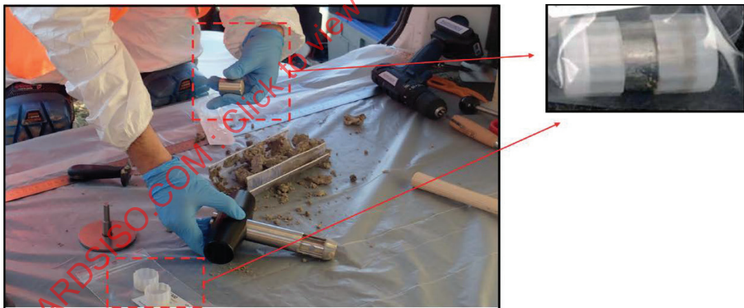
Figure 10 — Sampling with a soil corer containing a metal coring ring 16 ml
