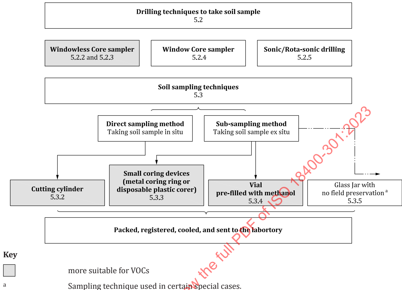
Figure 3 — Drilling and sampling techniques
