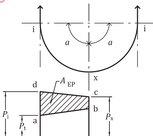
Figure 3 — Tensile force loss of prestressing steel due to setting (b)
