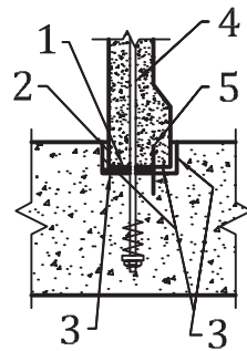
a) Prestressing bar fixed in the base slab (the bottom wall is not always thickened)
