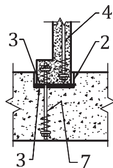
c) Anchor used prestressed bar
