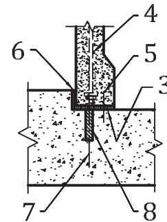
b) Anchor used with rebar (vertical structure of the tank wall is prestressed concrete)
