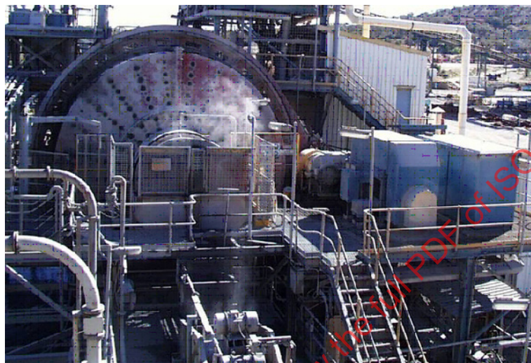
Figure C.1 — Mill drive train misalignment
