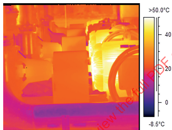
Figure 2 — Multiple machines (pump sets) comparison thermogram
