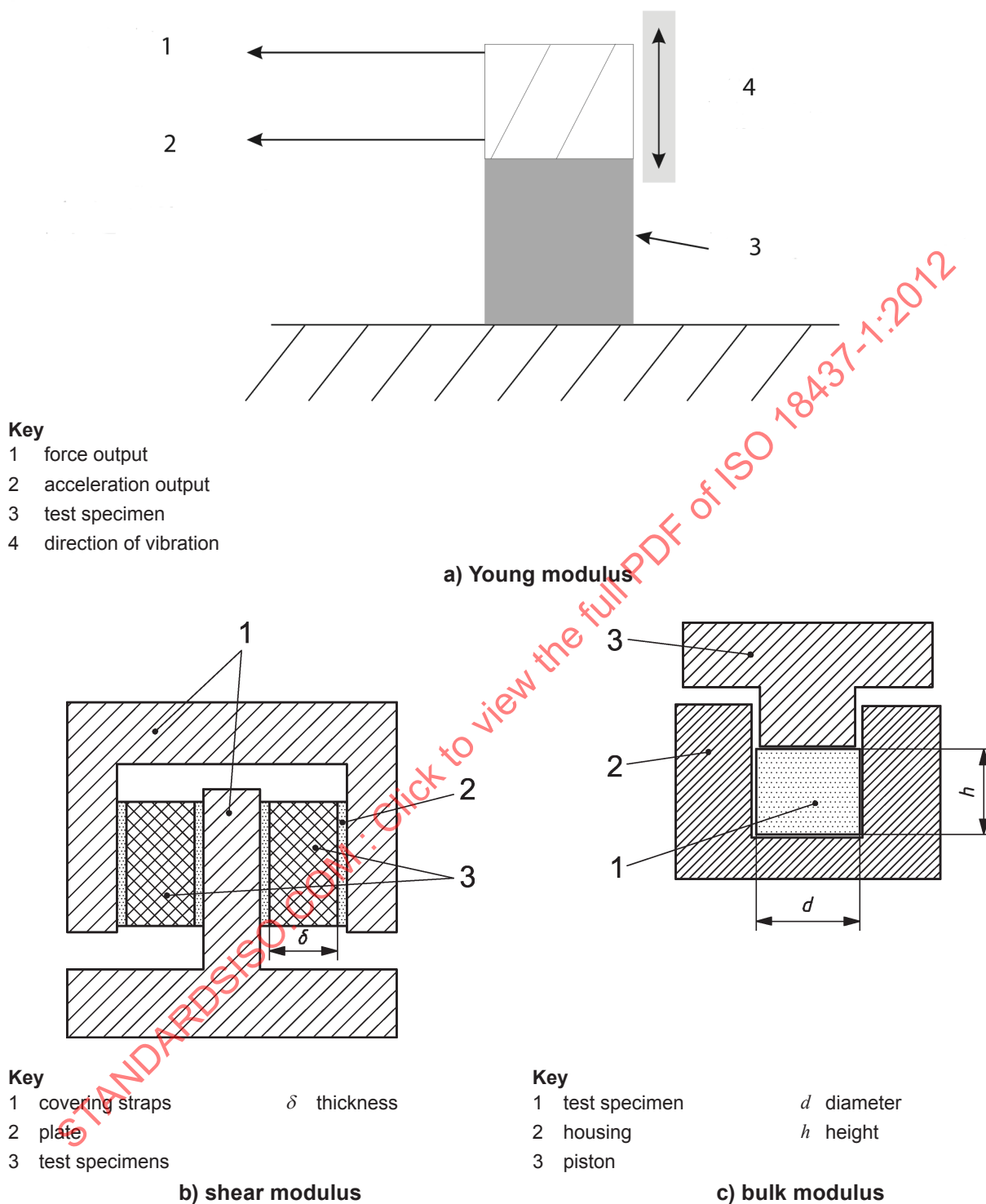
Figure 3 — Schematic diagrams of dynamic stiffness methods
