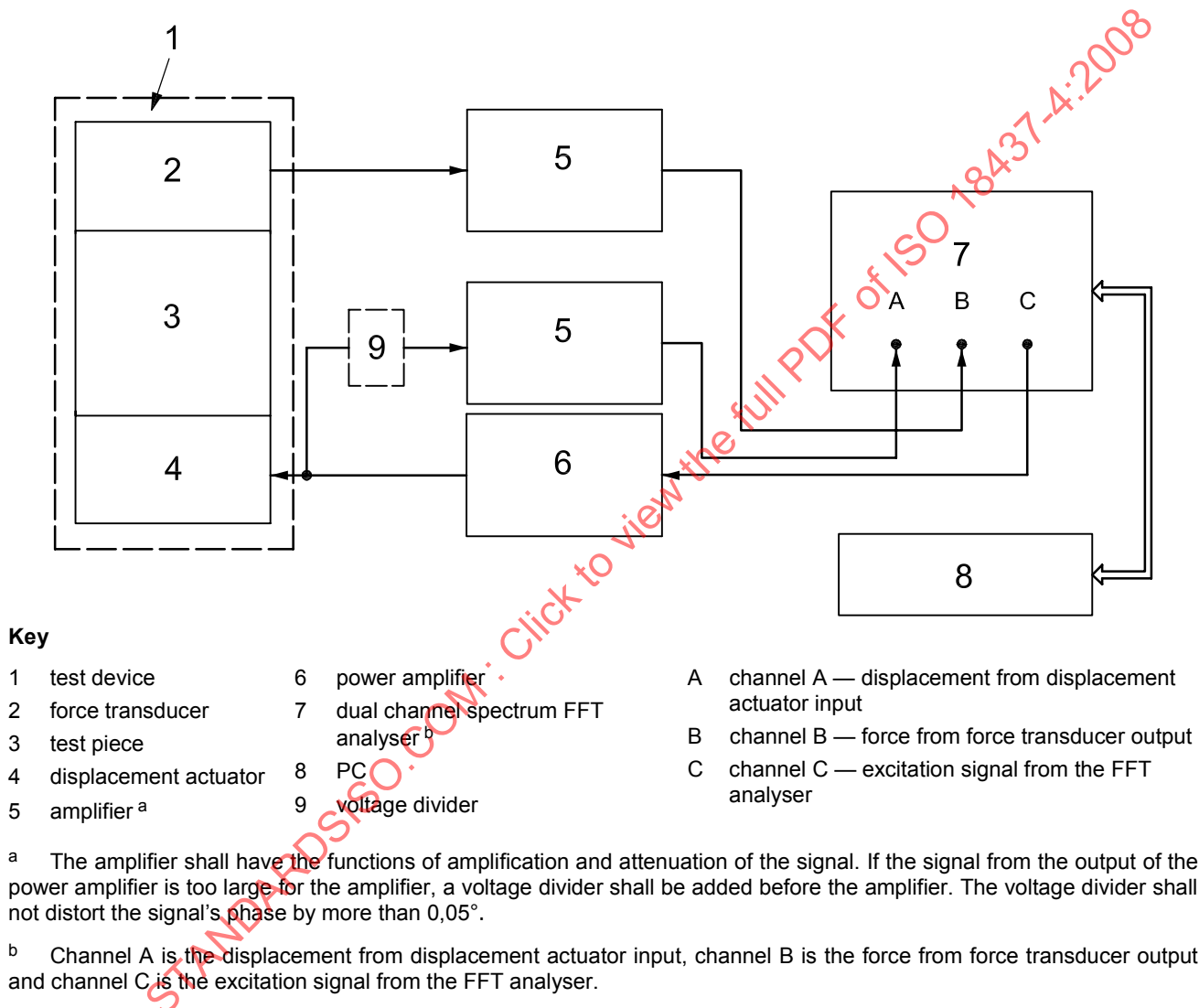
Figure 1 — Measurement set-up
