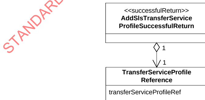
Figure 5-27: ASTSP-SR Message Structure Class Diagram
