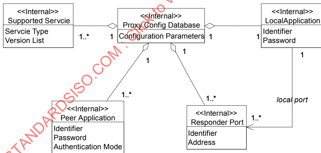
Figure 2-5: Configuration Database of the Proxy
