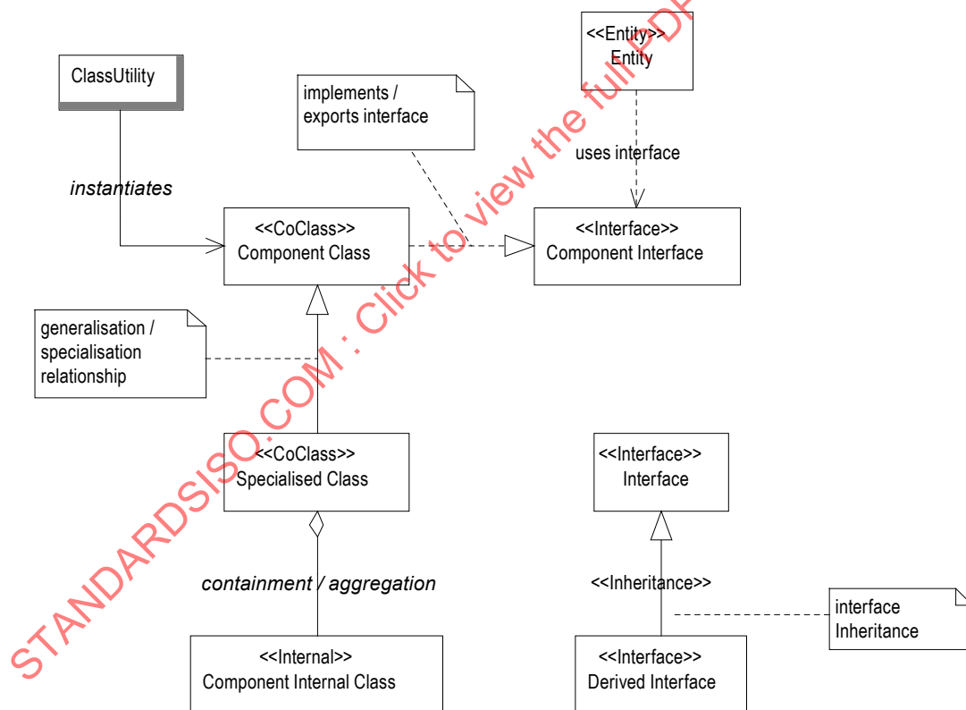
Figure 2-1: UML Stereotypes Used in This Recommended Practice
