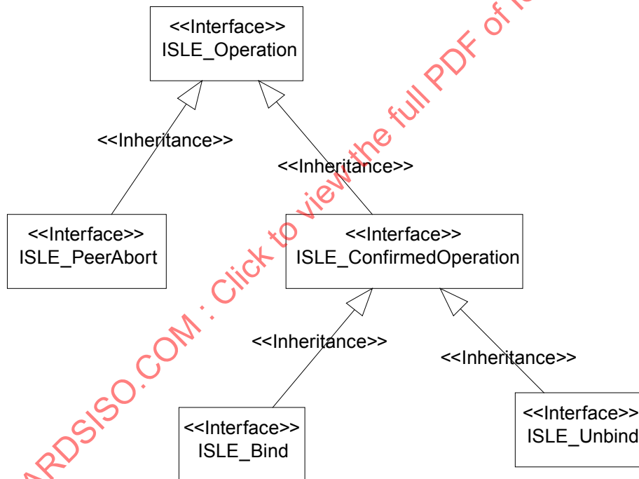
Figure 2-13: Operation Object Interfaces for Common Association Management
