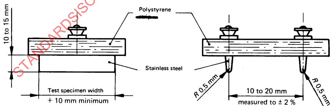
FIGURE 2 — Potentiometric electrodes
