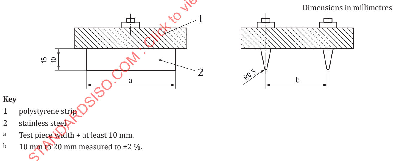
Figure 2 — Potentiometric electrodes
