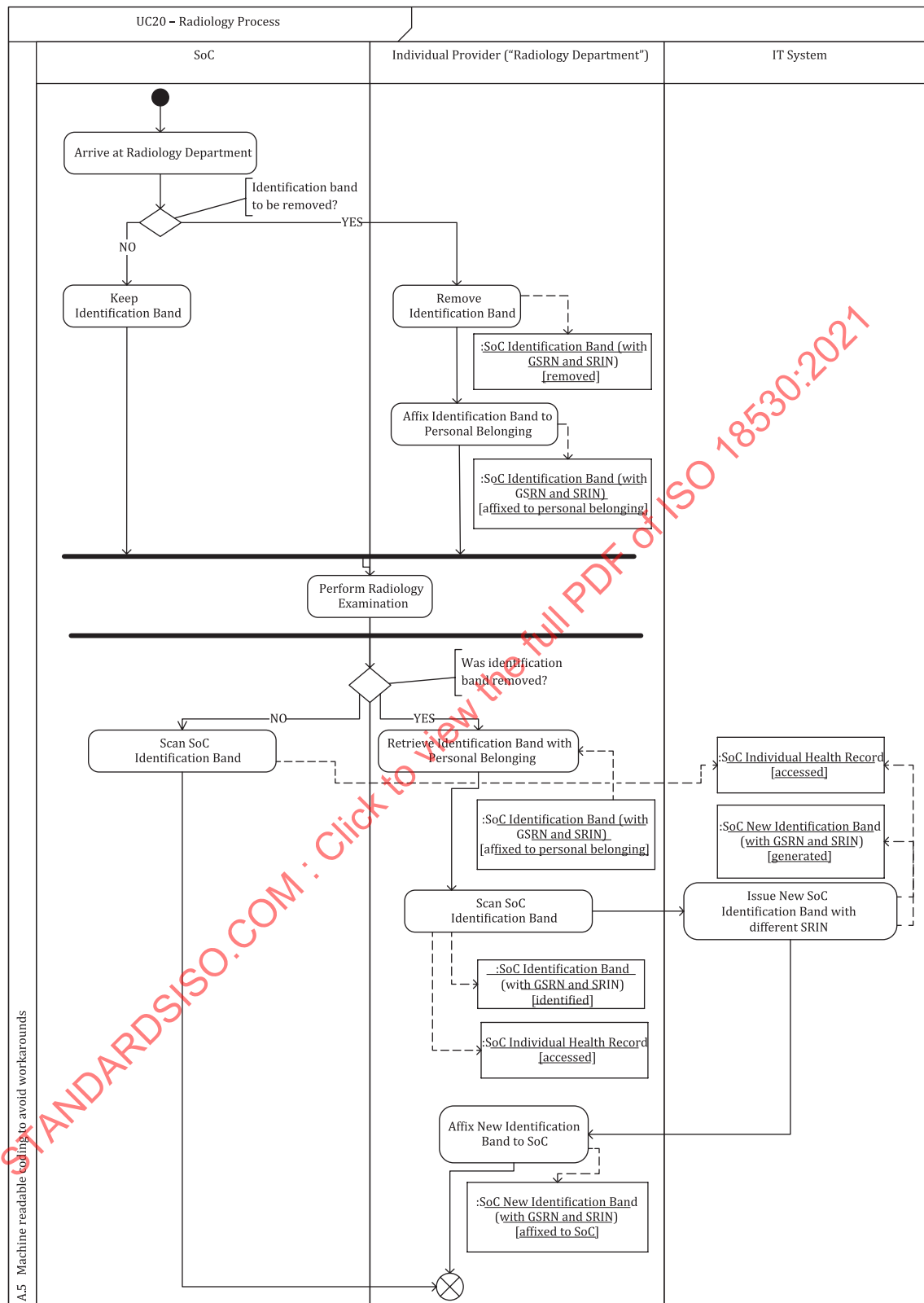
Figure A.4 — UC 19 and UC 20 Process flow
