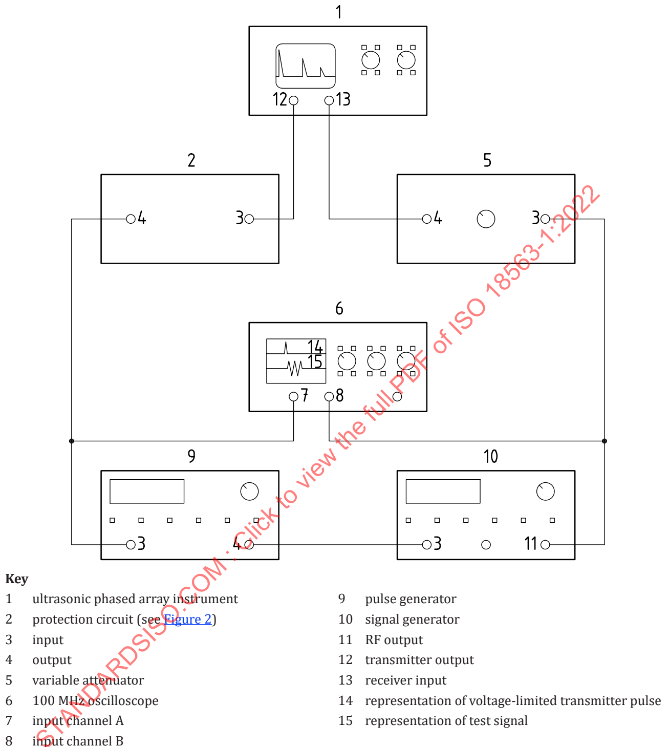
Figure 3 — Setup for measuring stability after warm-up time and against temperature
