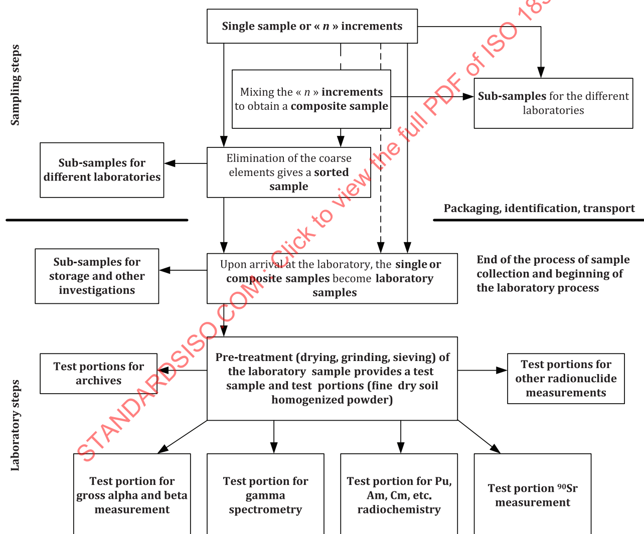
Figure 1 — Diagram of the evolution of the sample characteristics from the sampling site to the test laboratory
