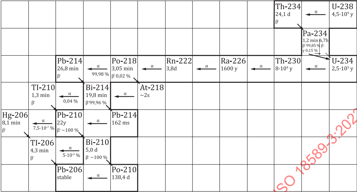
a) Uranium/radium ( A = 4n + 2 )
