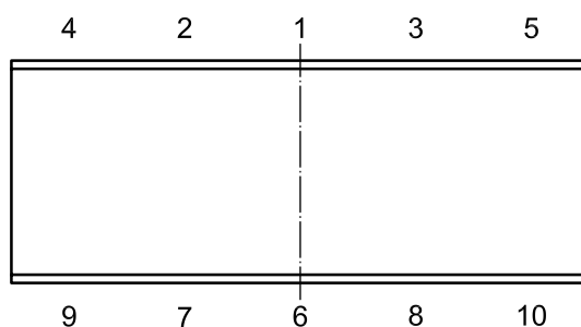
Figure 3 — Joining sequence for H-specimens
