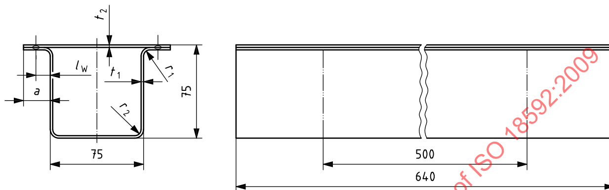
Figure 10 — Single-hat specimen
