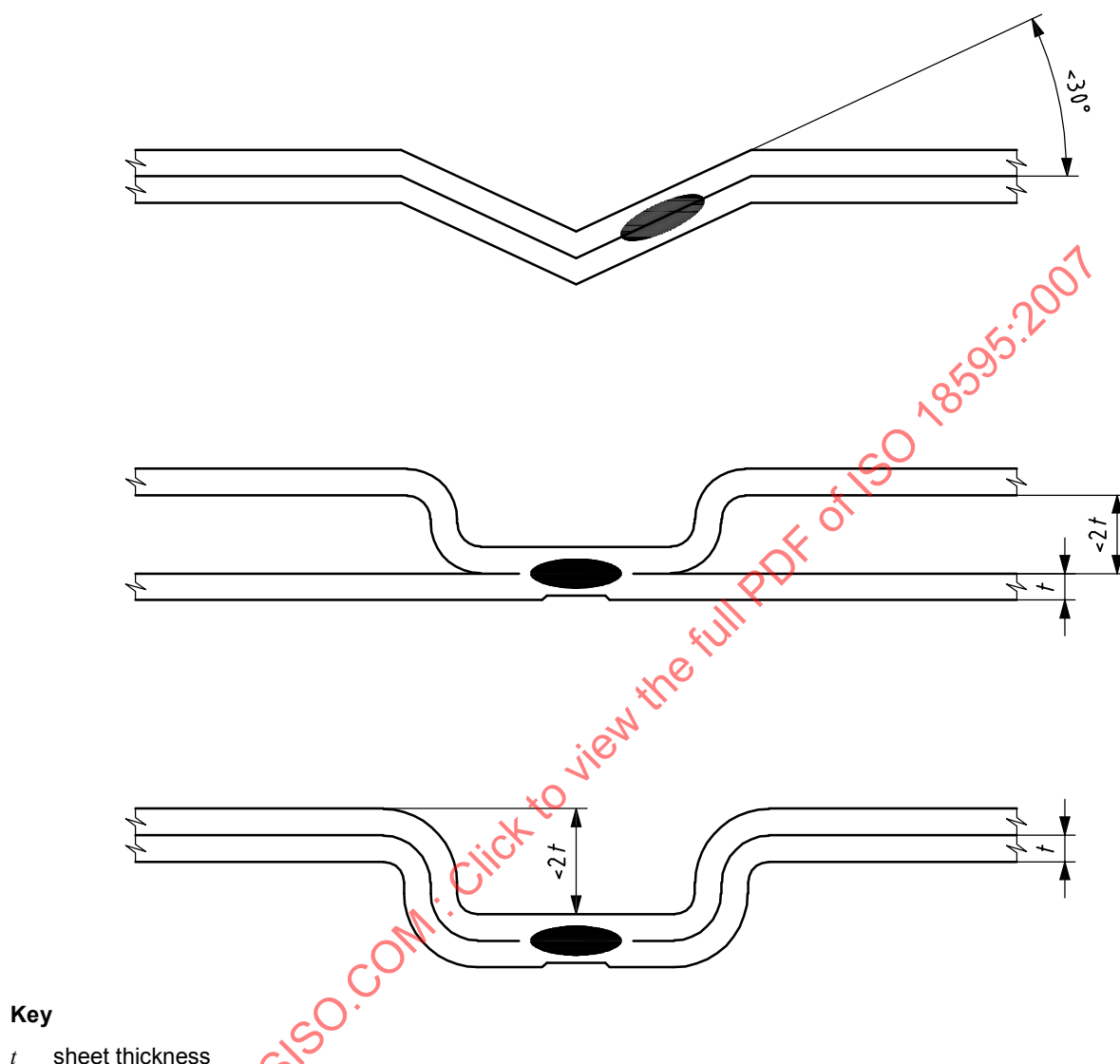
Figure 5 — Maximum permissible distortion of sheet
