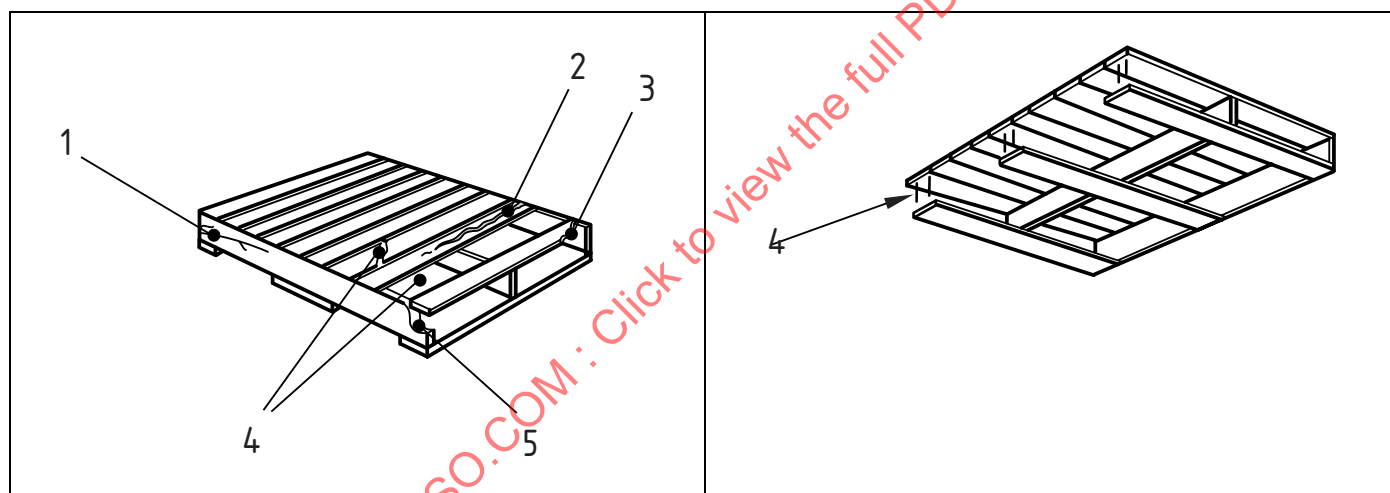
Figure C.1 — Criteria for which a 2-way stringer (bearer) pallet cannot be reused
