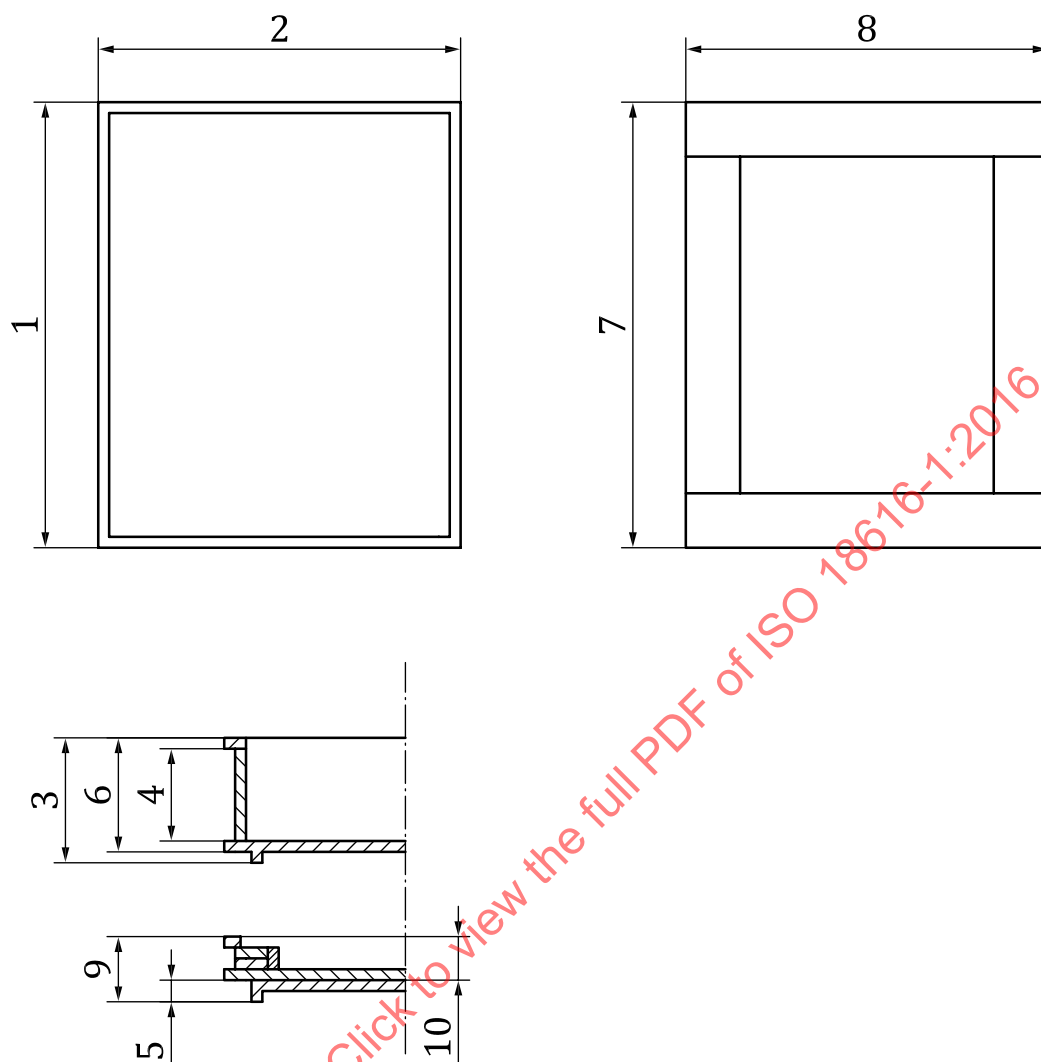
Figure 4 — Foldable box without plan view dimensions changed (1 = 7 and 2 = 8)
