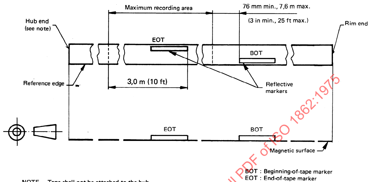
FIGURE 3 — Reflective markers and recording area
