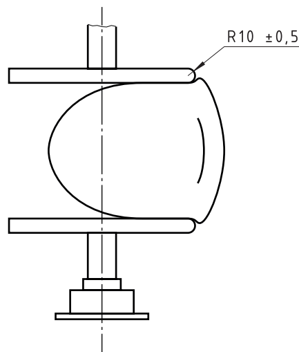
Figure 2 — Lateral crushing
