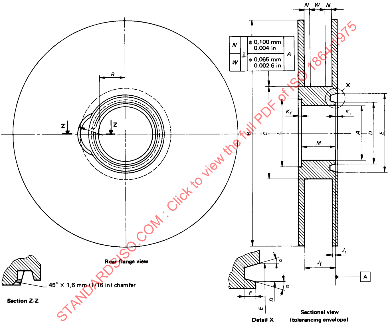
FIGURE 3 – Tape reel
