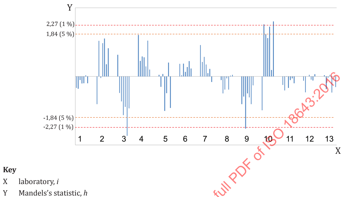
Figure A.1 — Mandel's inter-laboratory consistency statistic, h , grouped by laboratories
