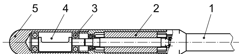
a) Eccentric-type immersion vibrator
