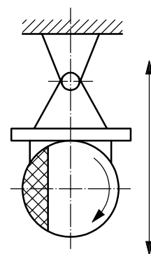
b) External vibrator fixed on hinge
