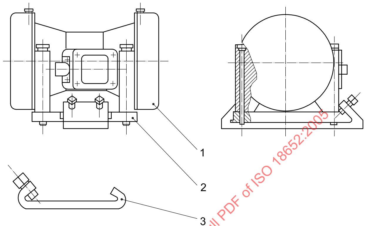
a) Dovetail guidance form
