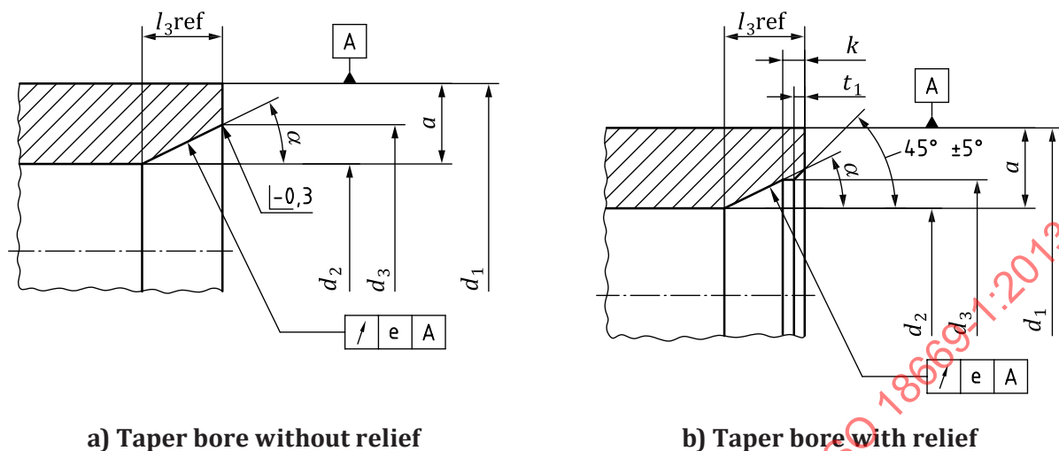
Figure 16 — Tapered bore configurations
