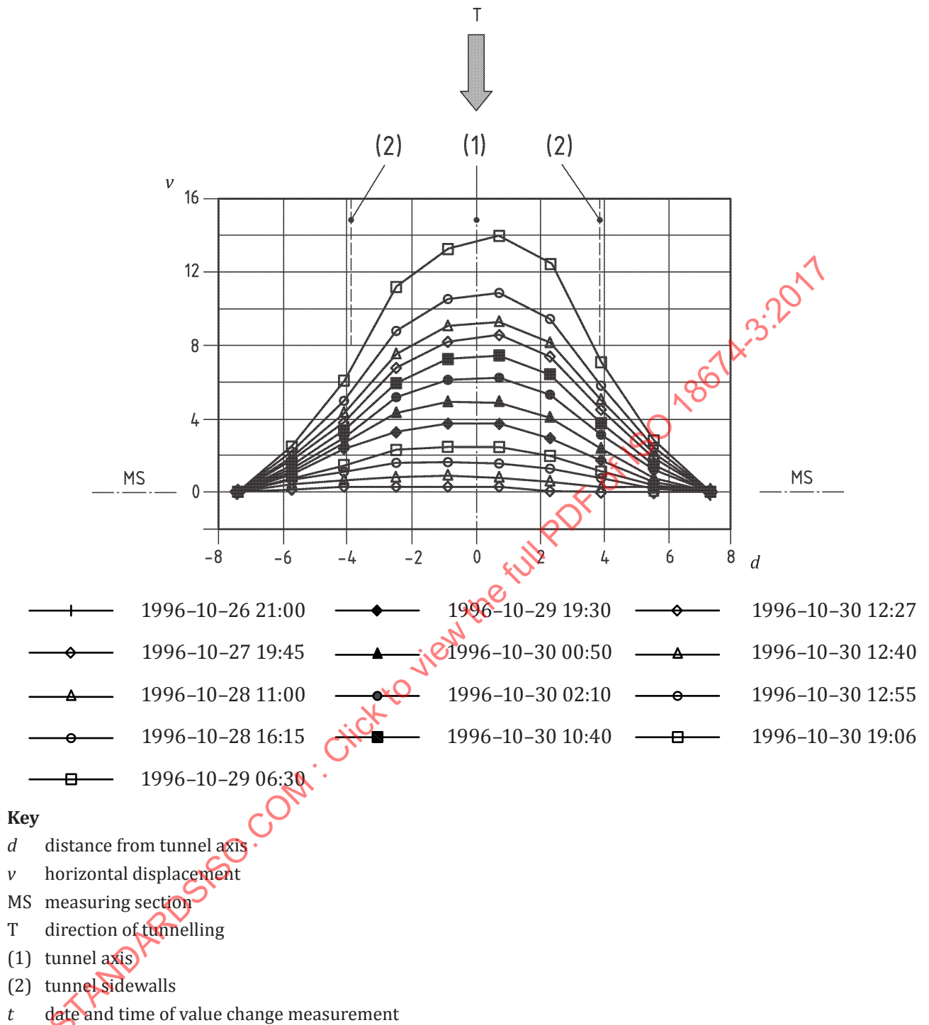
Figure E.3 — Horizontal section showing the horizontal displacements of the ground ahead of tunnelling and displacement profiles at various points in time of the tunnel face approaching the measuring section
