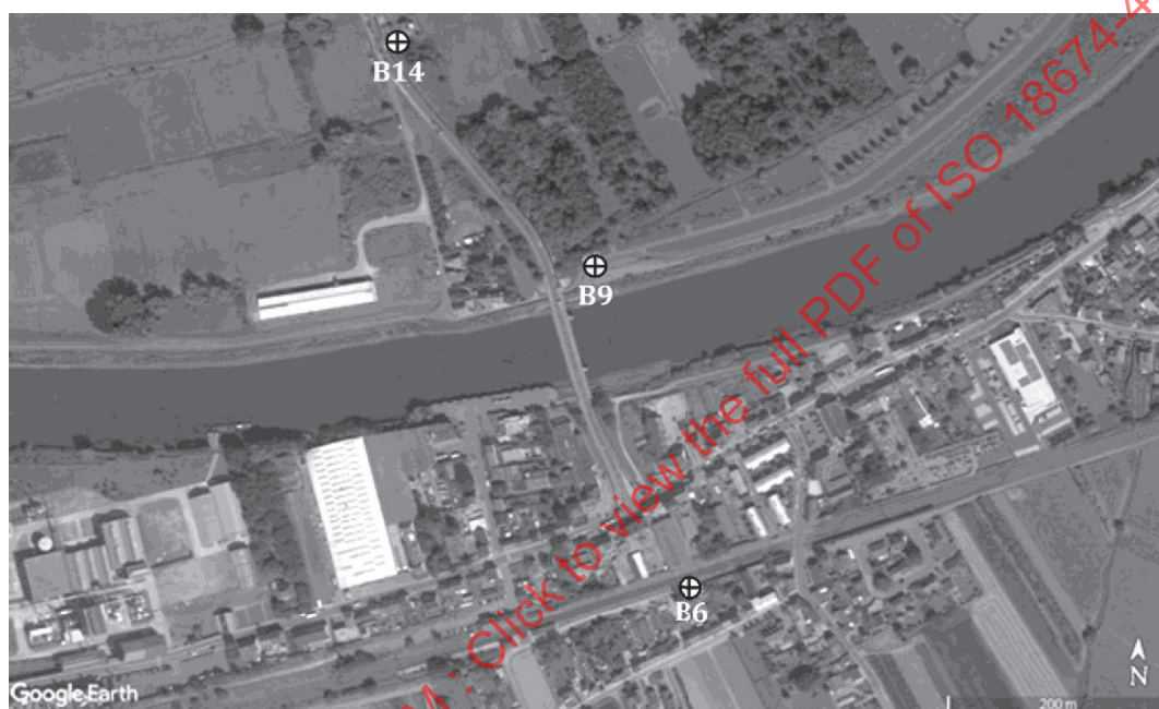
Figure G.1 — Location of the open standpipe piezometer boreholes B6, B9 and B14
