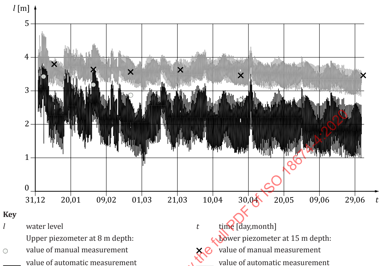
Figure G.2 — Open standpipe piezometer P9 — Tidal influence: comparison between automatic and manual measurements
