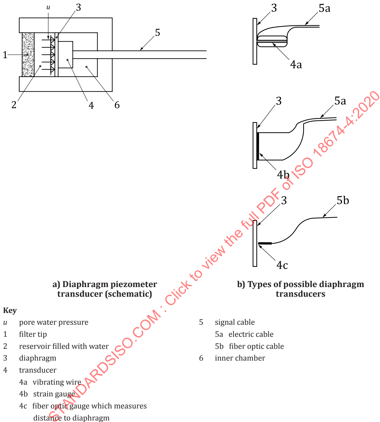
Figure 3 — Diaphragm pressure transducers of different types of closed piezometer systems
