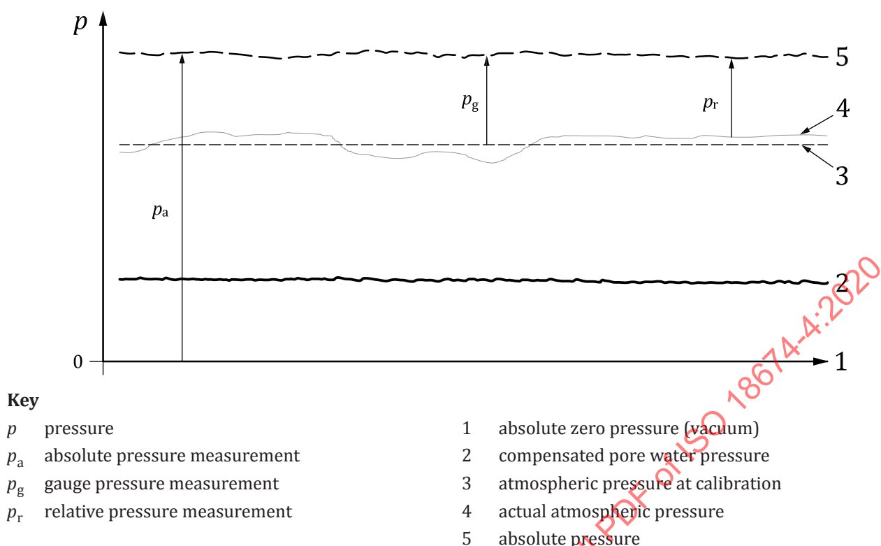
Figure 6 — Absolute gauge and relative pressure measurements
