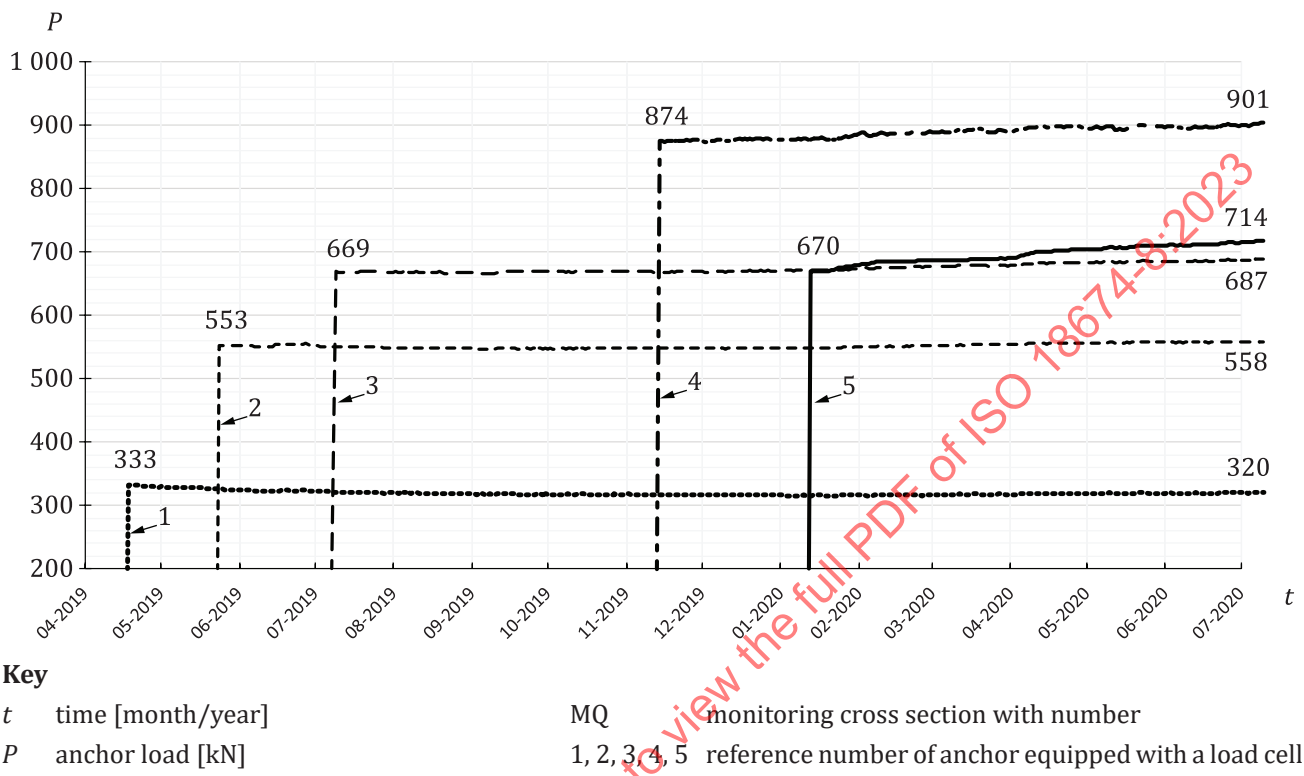
Figure B.9 — Measurements of anchor loads in section MQ 4.02
