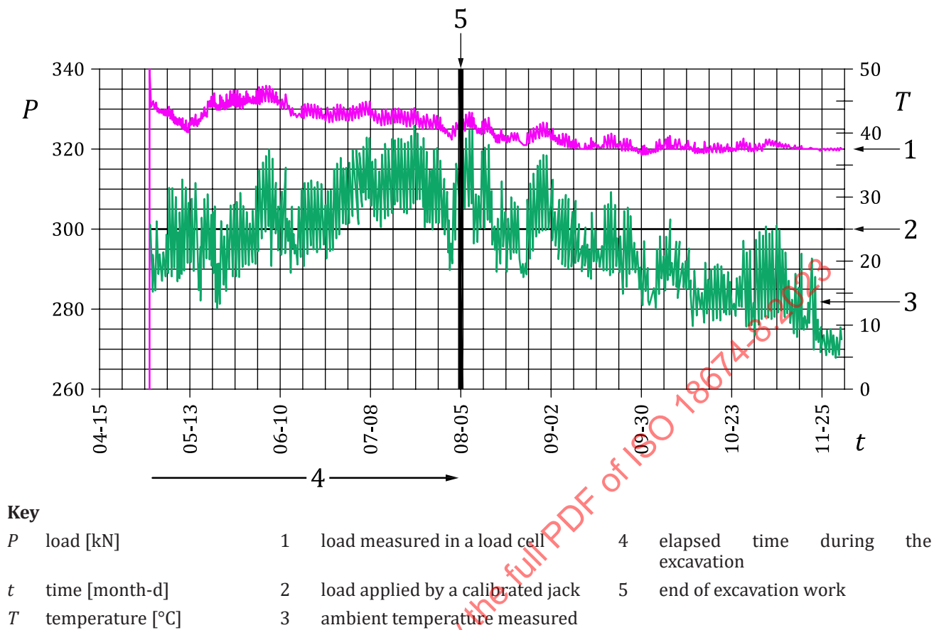
Figure B.4 — Load and temperature measurements for a period of eight months, during and after the excavation works
