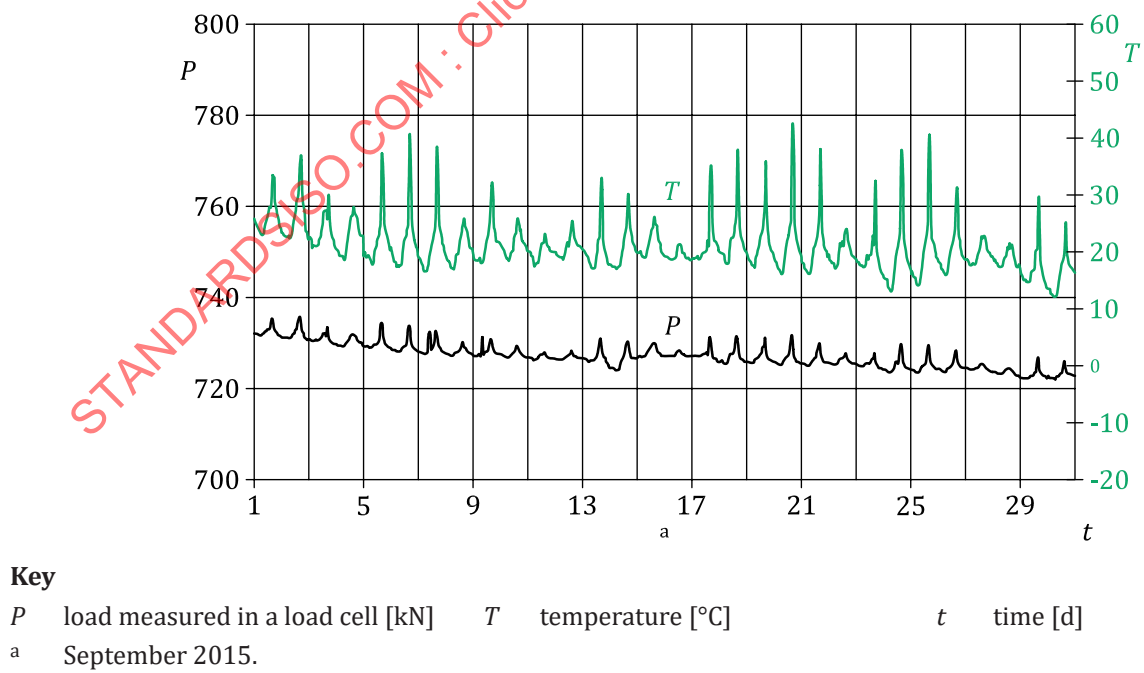
Figure B.5 — Evolution of load and temperature during one month
