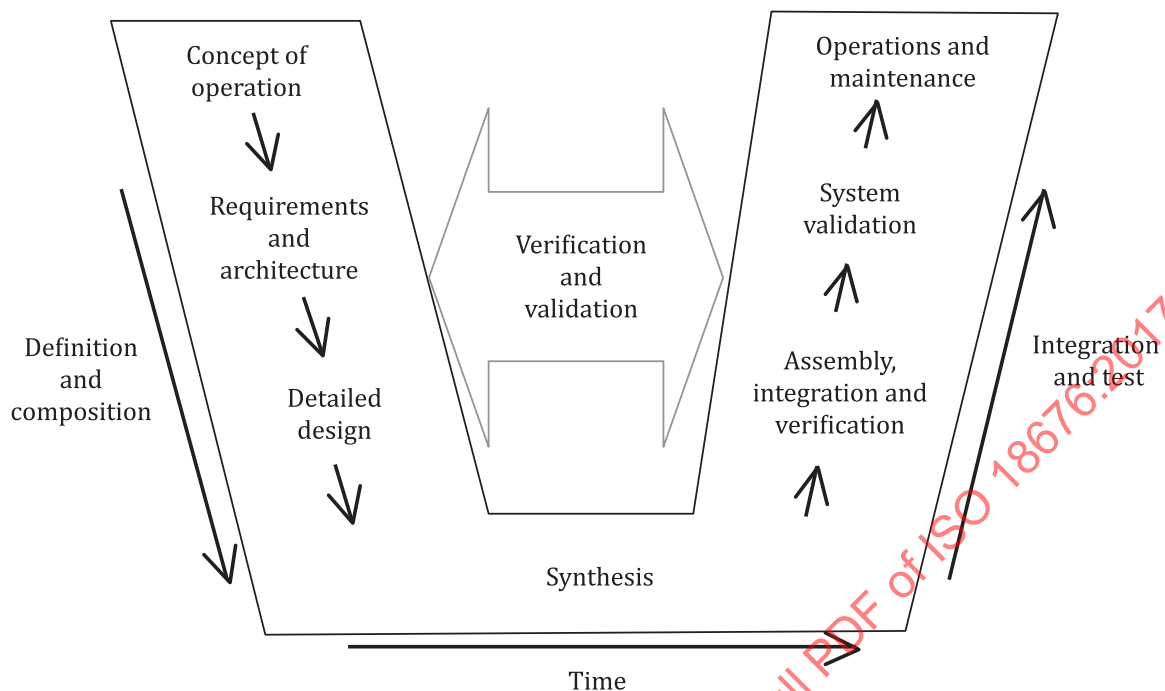
Figure 1 — Systems engineering V model
