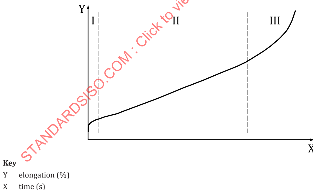
Figure C.1 — Typical HMPE creep curve
