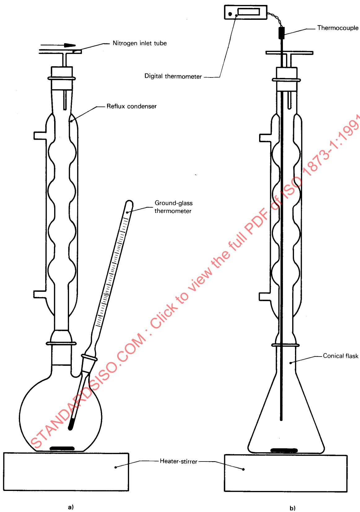
Figure A.1 — Apparatus for preparation of test solution
