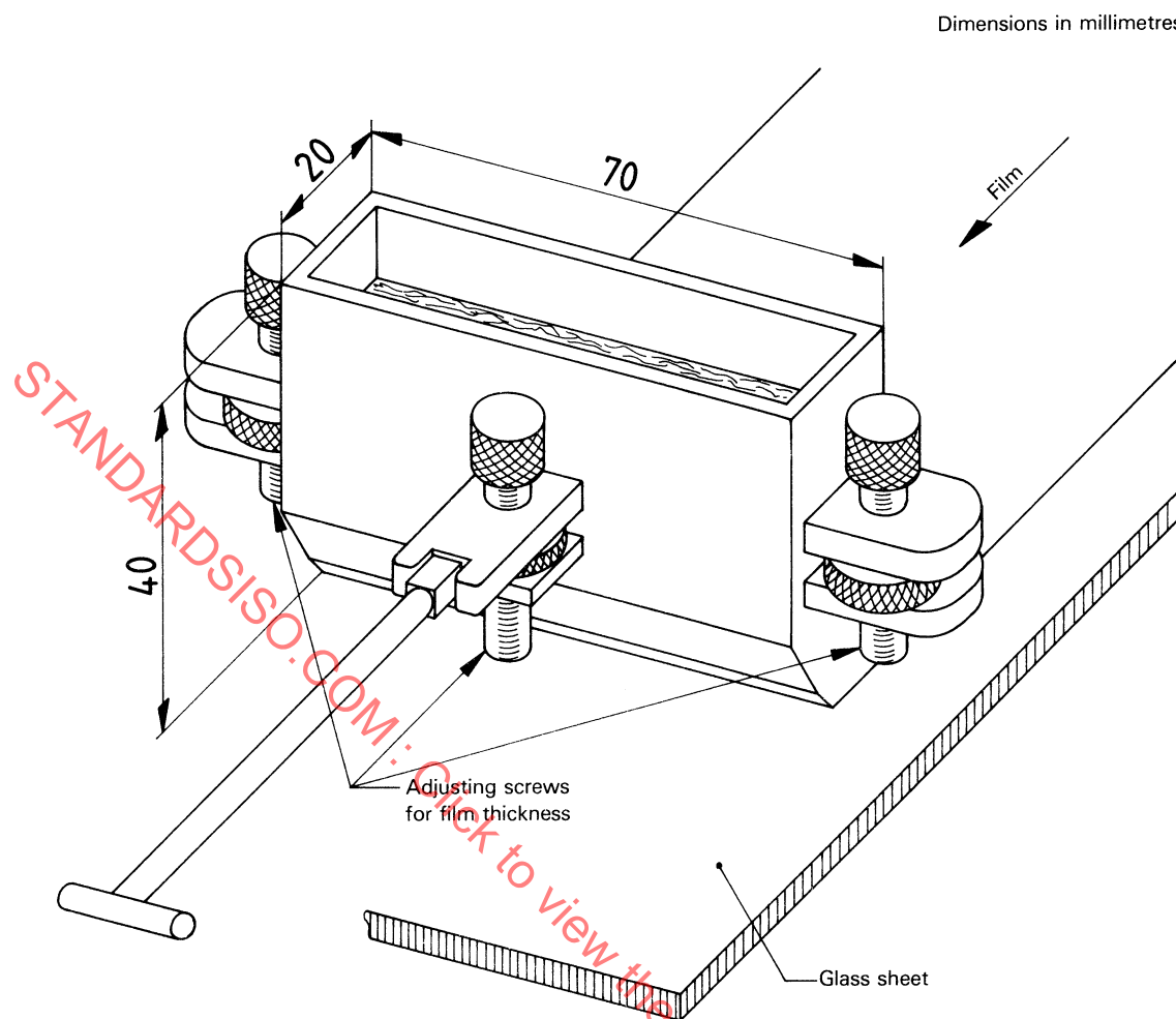
Figure — Suitable type of film casting device
