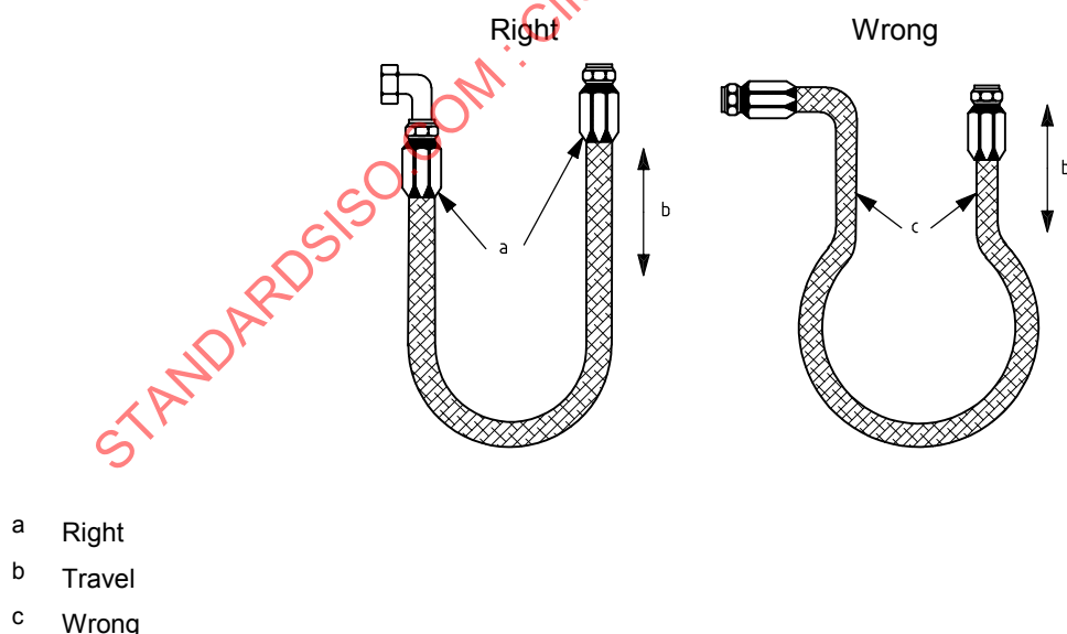
Figure A.1 — Metallic flexible hose — General installation guidelines
