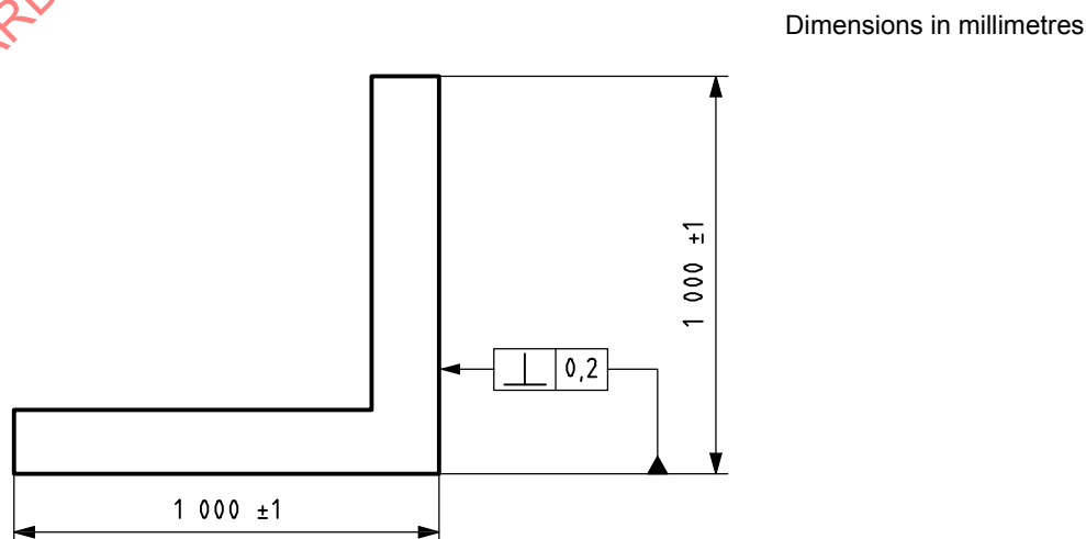
Figure 1 — Accuracy requirements of mechanical square
